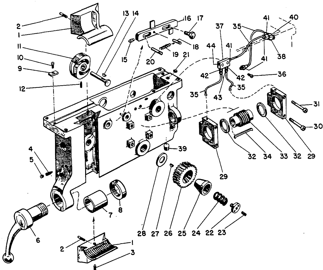
Figure 11. Apron Assembly (Rear) 15'' and 18''
