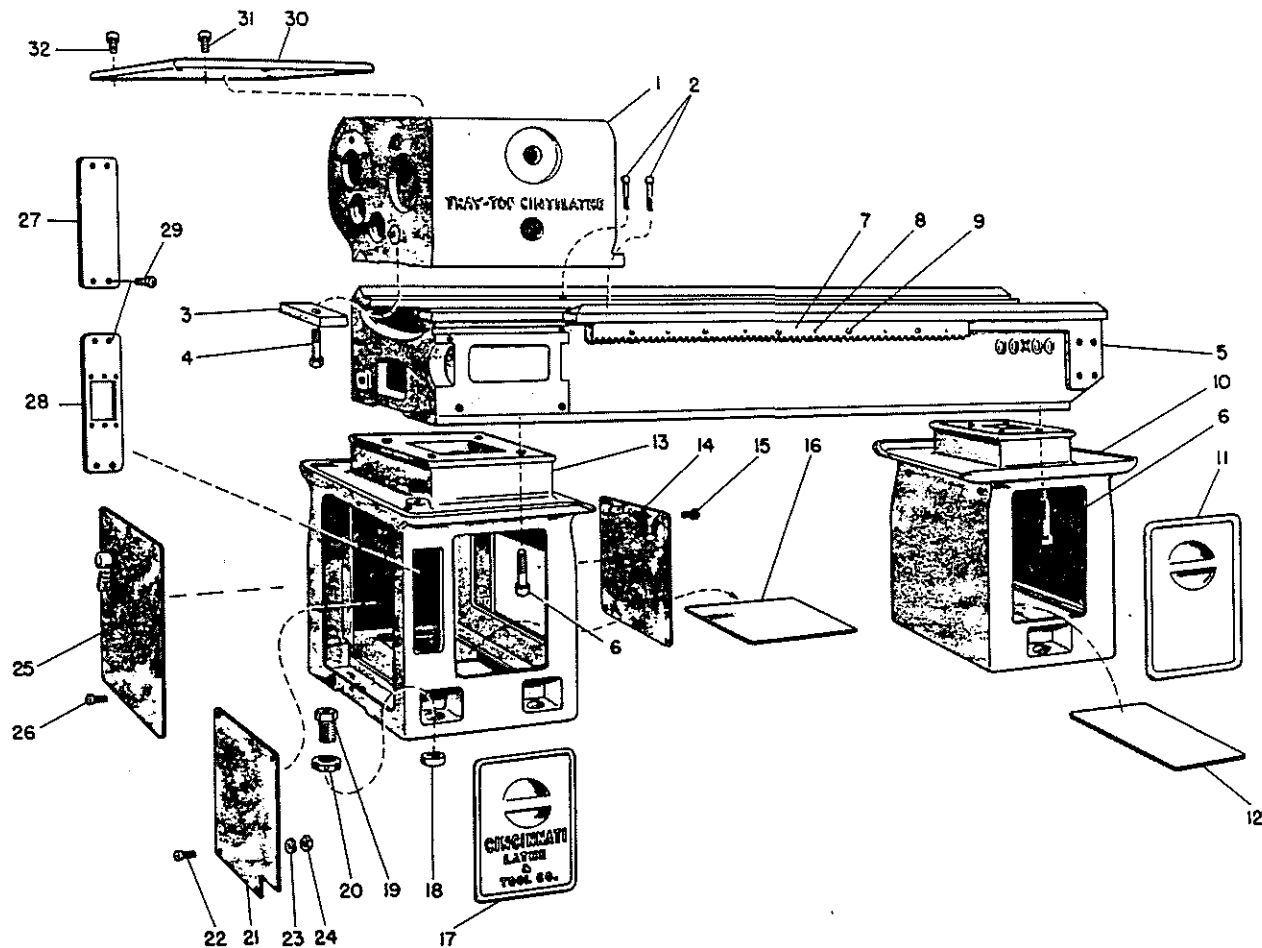
Figure 1. General Assembly
