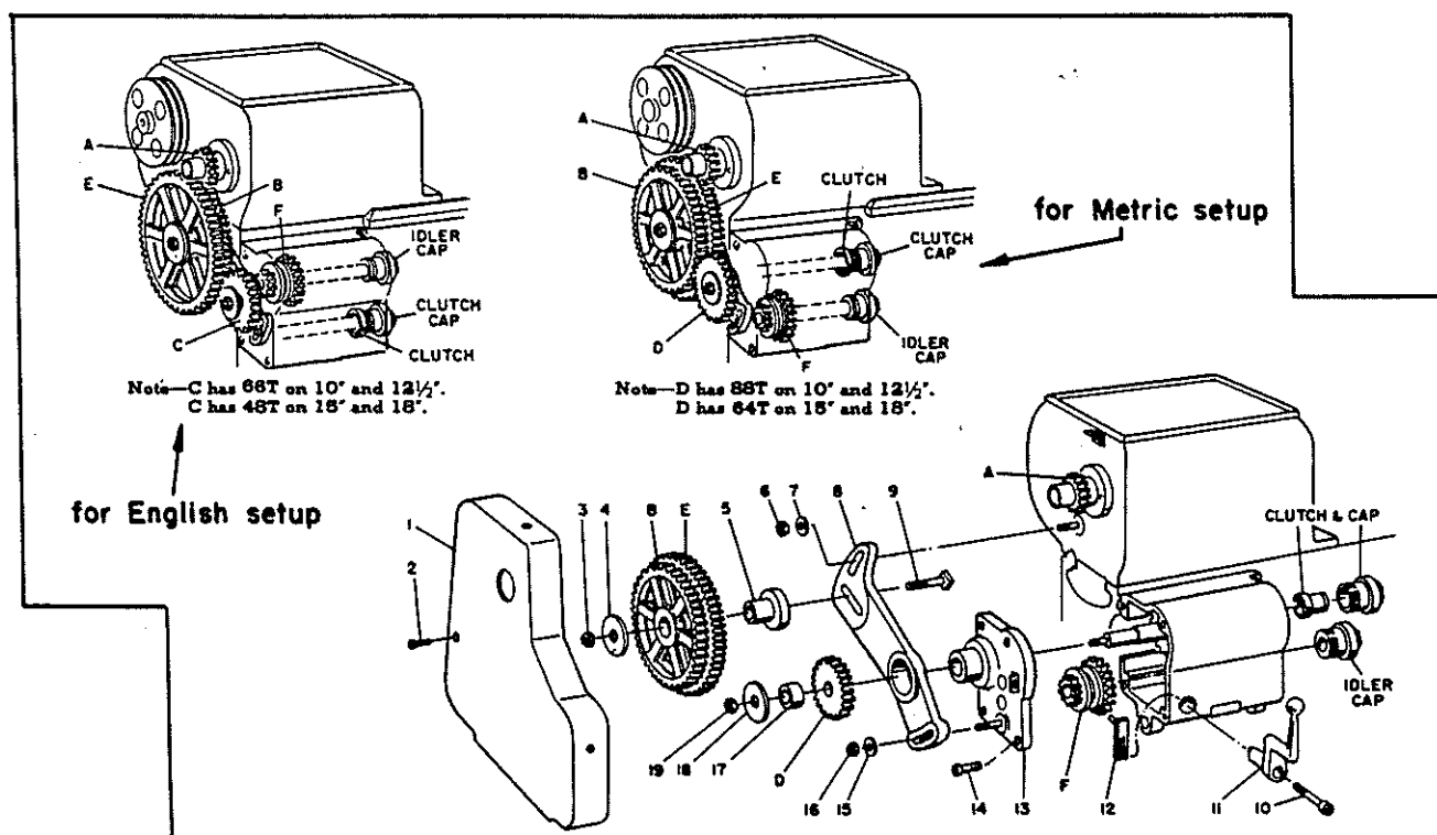
Figure 3-11. Metric Conversion
