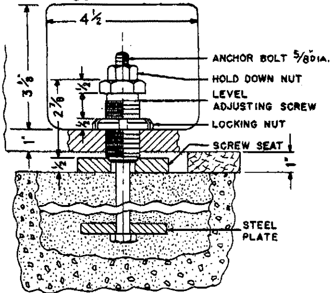
Figure 3-6. Anchoring Machine
