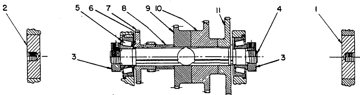
Figure 5-9. Intermediate Shaft
