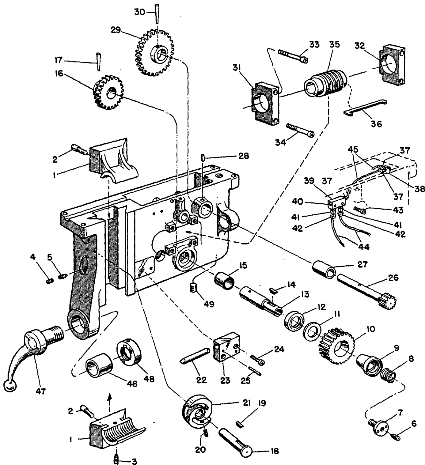
Figure 9. Apron Assembly (Rear) 10" and 12 1/2"
