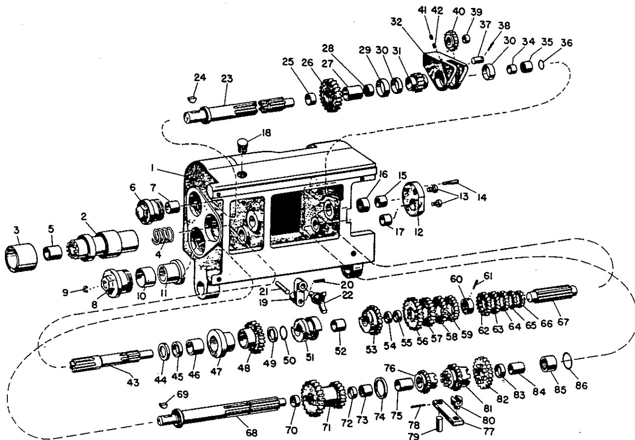
Figure 13. Quick Change Box Assembly (Rear)
