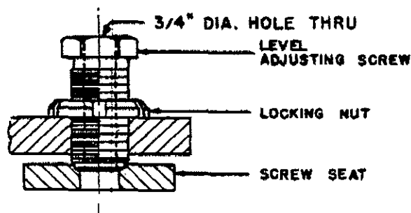
Figure 3-5. Leveling Jack Assembly
