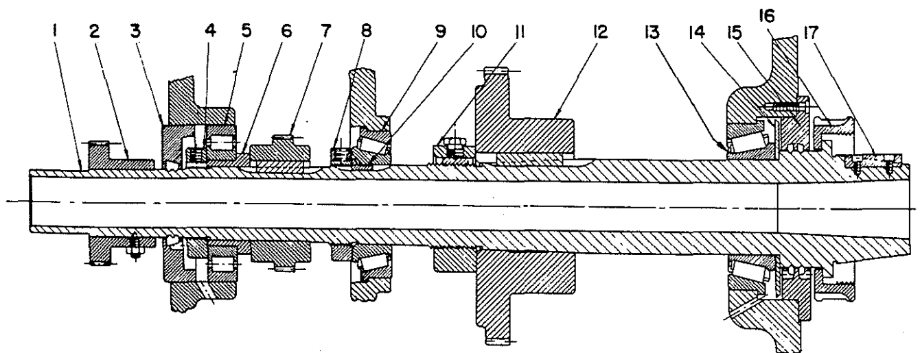
Figure 5-6. Headstock Spindle
