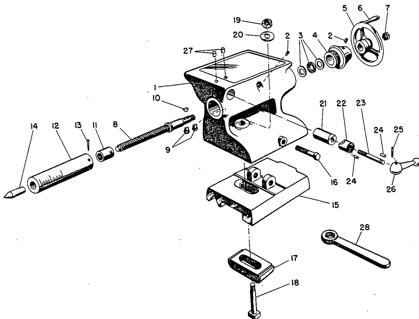
Figure 6. Tailstock Assembly
