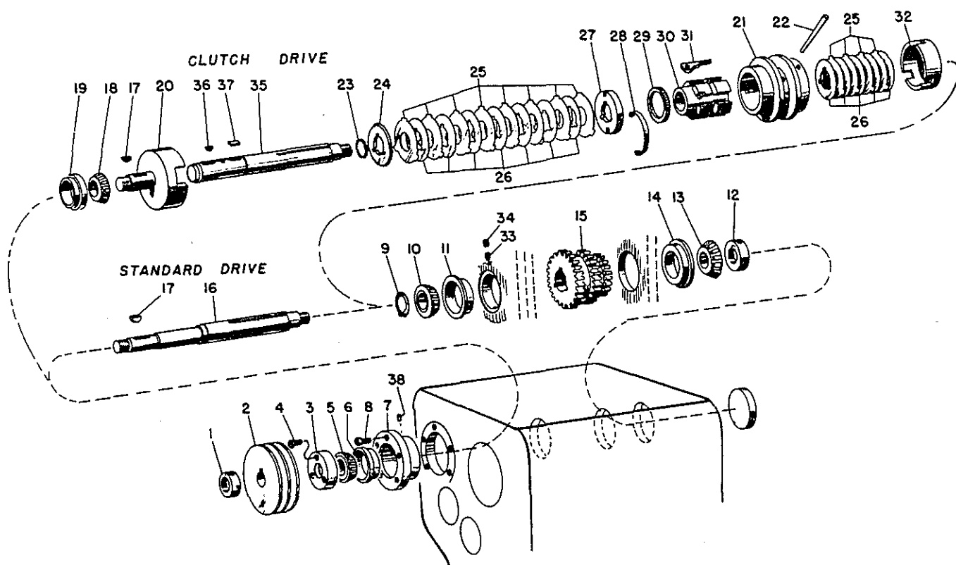
Figure 5. Pulley Drive Shaft Assembly
